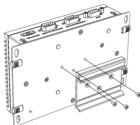
DIN-Rail Mount (Optional)
